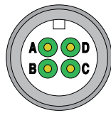
4 Pin mini-MIL
