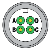
4 Pin mini-MIL
