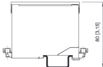
Mounting on DIN rail NS 35/15
