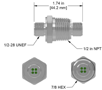
4 Pin mini-MIL to 4 Pin mini-MIL Bulkhead Feedthrough, 0.5 in. (12.7 mm) NPT, Stainless Steel
